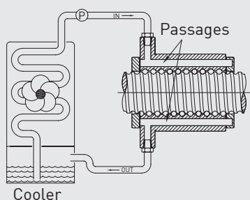
Fig. 8.2 Cool type I with cooler
