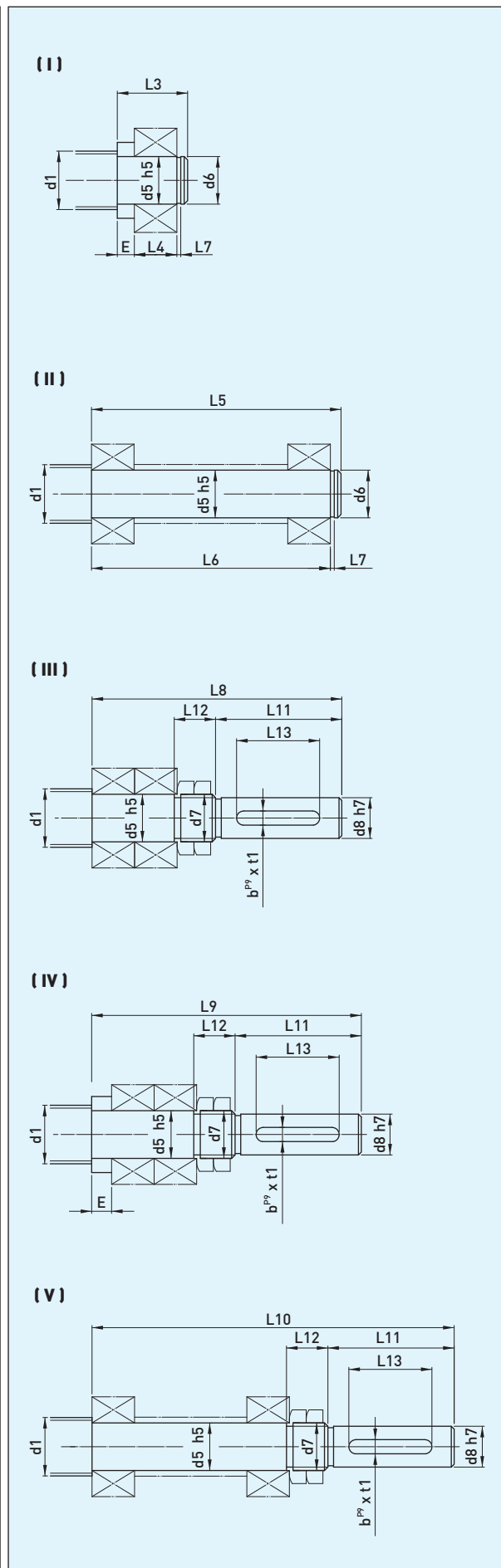
Fig 3.9 Configurations of spindle ends
