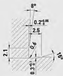
F0.6X0.3DIN509
