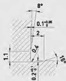
F0.4X0.2DIN509
