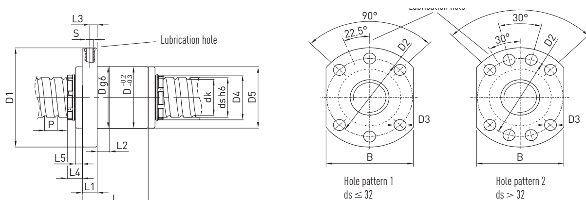
Fig. 10.5 Flange single nut DEB-x with Wiper K and V
