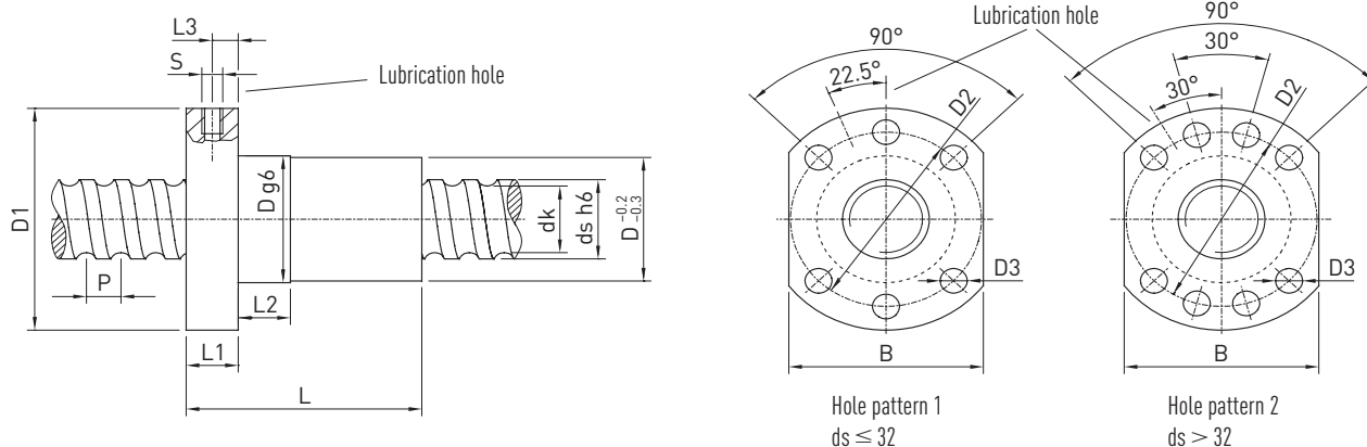
Fig. 10.4 Flange single nut DEB-x with Wiper N and F
