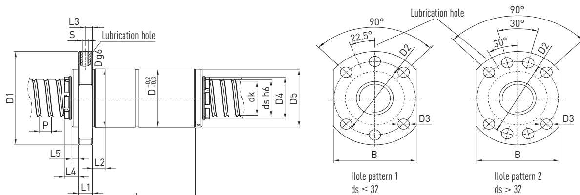
Fig. 10.7 Flange double nut DDB-x with Wiper K and V
