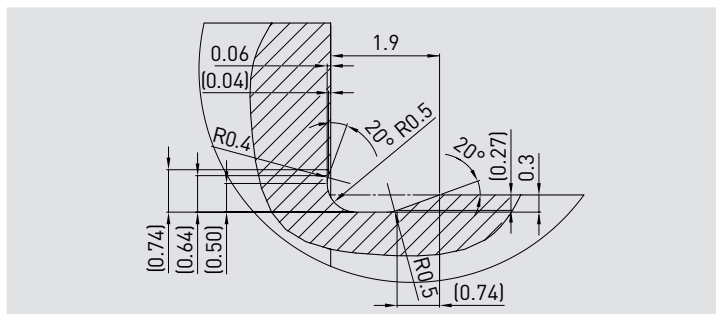
HIWIN recess 10002475
